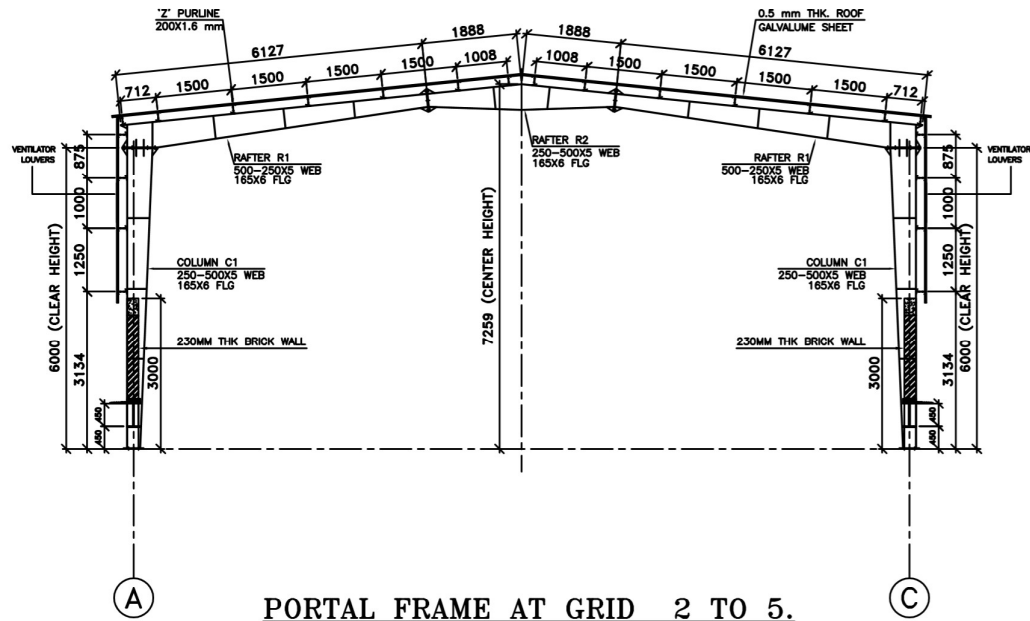
PORTAL FRAME AT GRID 2 TO 5.
