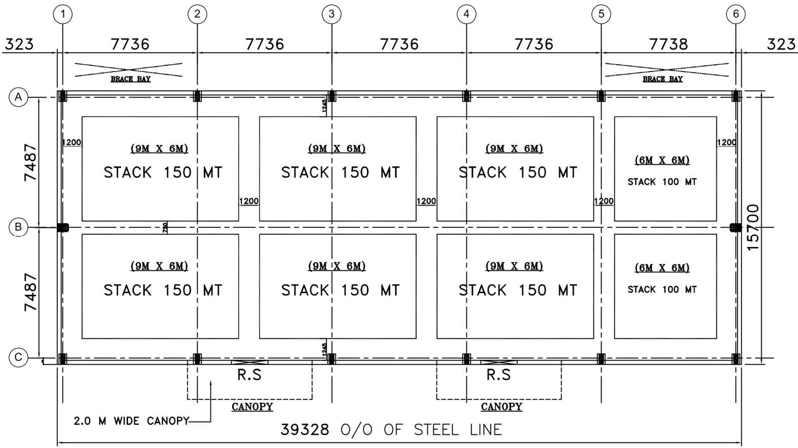
LAYOUT PLAN
