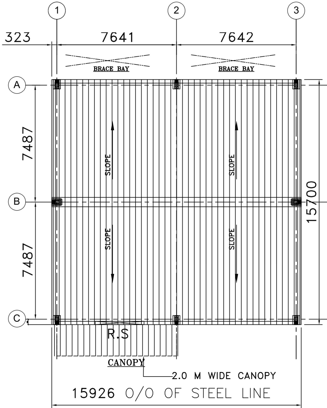
LAYOUT PLAN
