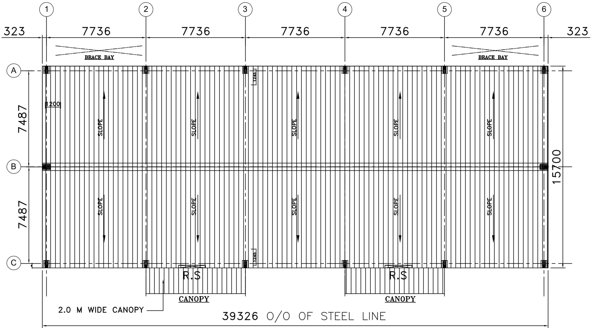
ROOF LAYOUT PLAN
