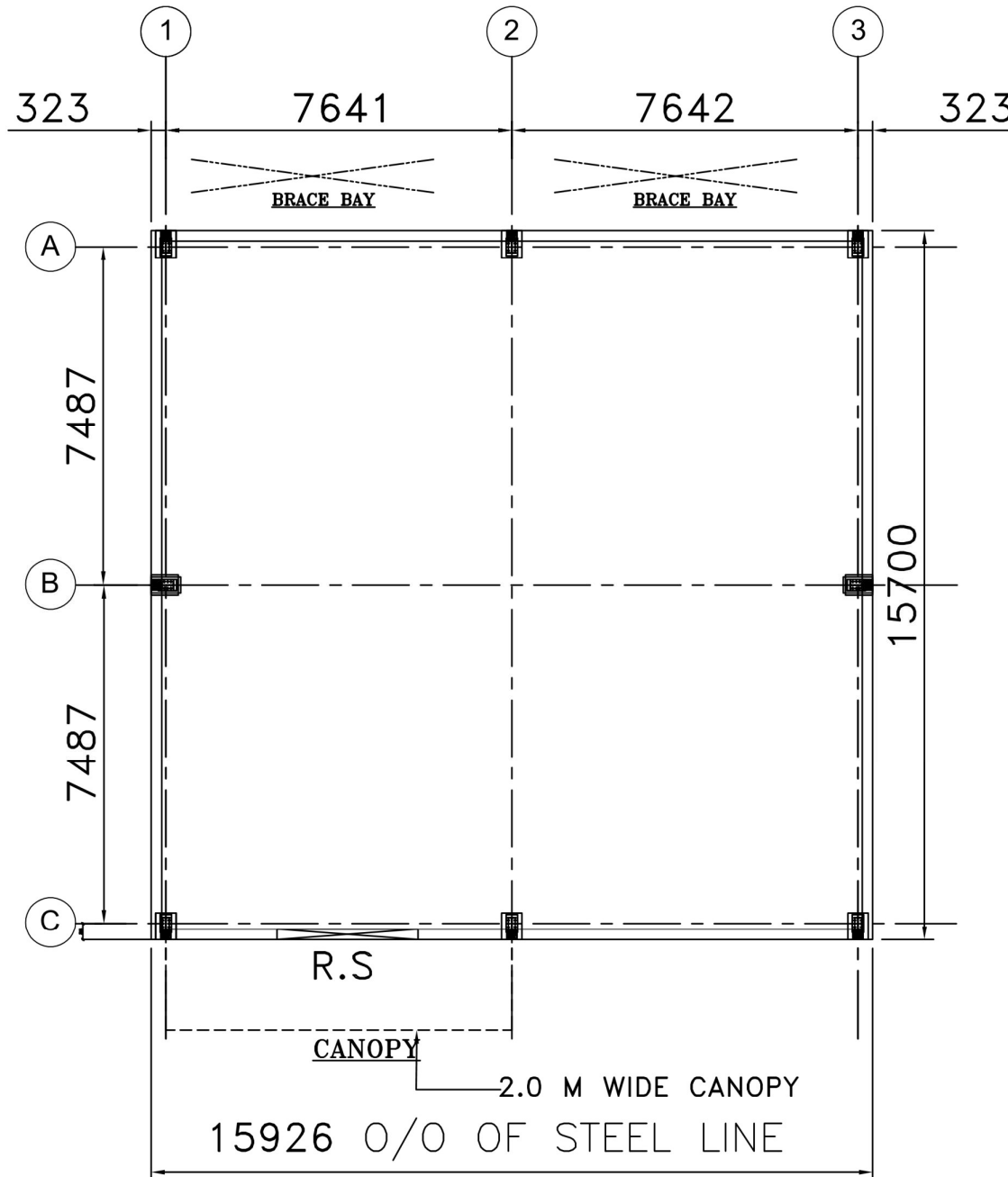
LAYOUT PLAN
