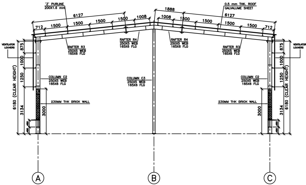
PORTAL FRAME AT GRID 1 & 6.
